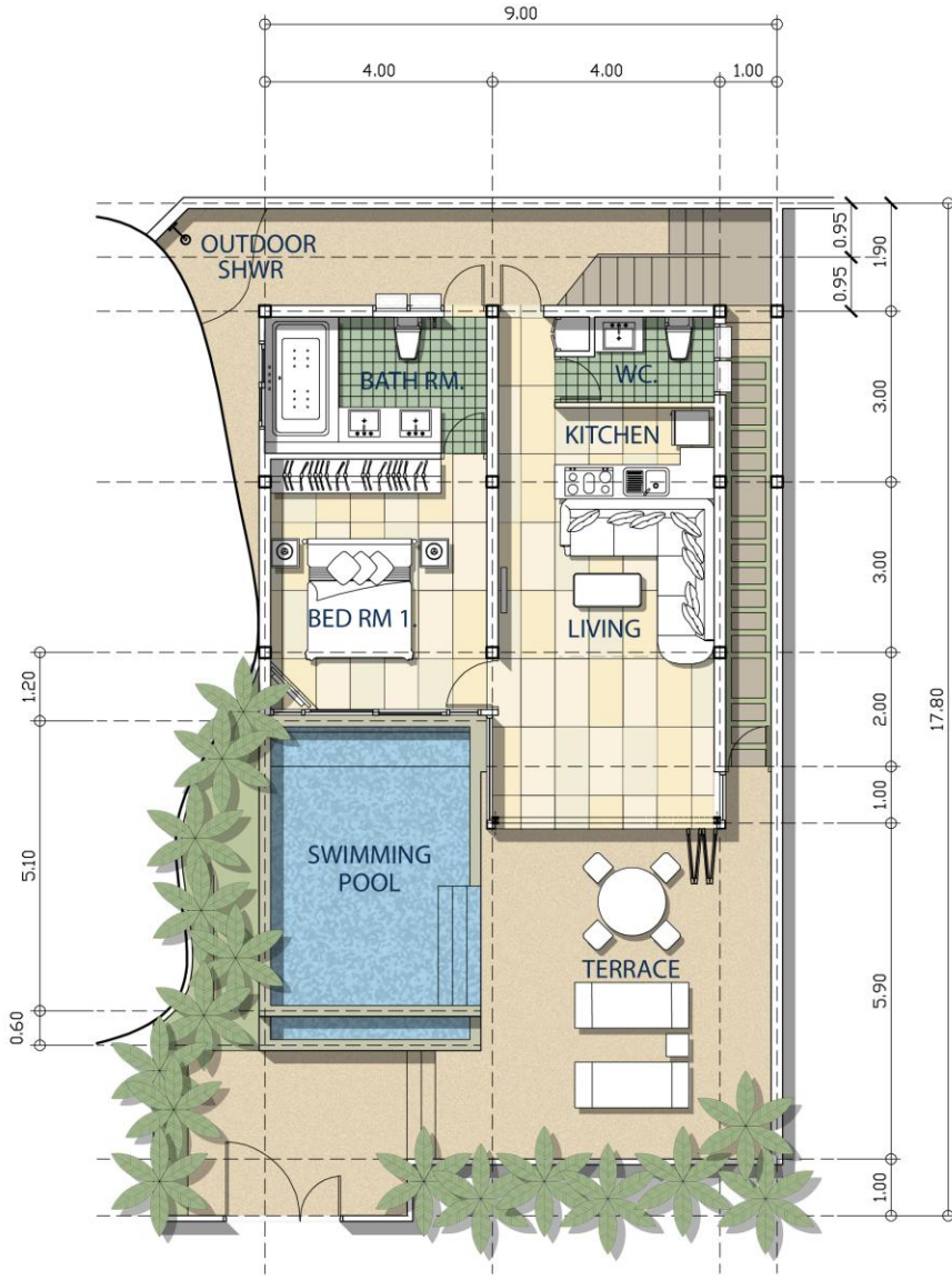
2 BED VILLA (TYPE A) GROUND FLOOR
